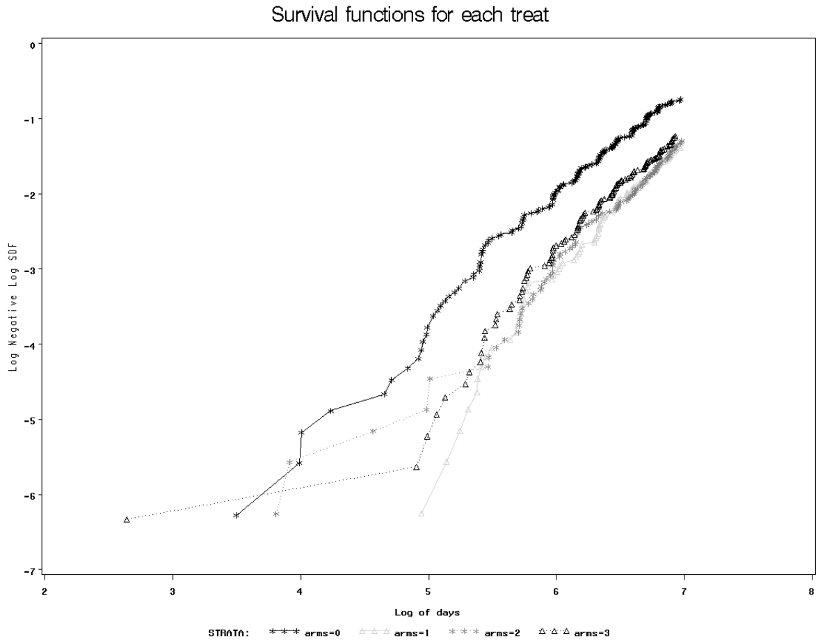
Fig. 1: ACTG 175 data. Log-negative-log survival functions of time to death for treatment 0, 1, 2 and 3, respectively.
